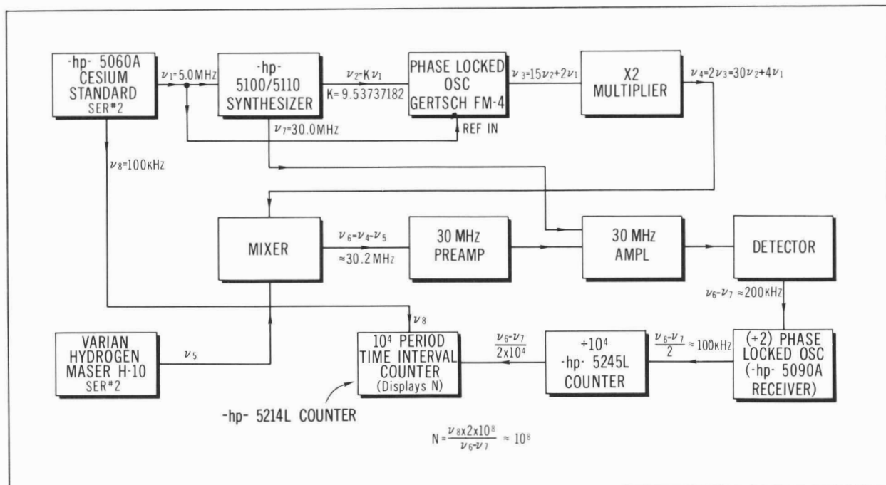
Fig. 1. Block diagram of equipment arrangement used to measure ratio of output frequencies of Cesium Beam Frequency Standard and Hydrogen Maser.
