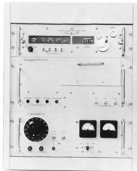
Fig. 4. Panel view of one of "atomic" clocks used in experiment. Cesium standard in middle drives electronic clock (top) which integrates standard frequency and also produces very accurate electrical "ticks" based on driving frequency. Power supply unit at bottom provides for operation from a range of ac and dc voltages.
