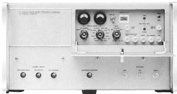
Fig. 7. Front view of Cesium Beam Frequency Standard. Cesium beam standards utilize a quantum-mechanical effect to produce ultra-stable frequencies. Two standards were combined with electronic clocks and power supplies to form an "atomic" clock with stabilities of a few parts in 10^{12} .
