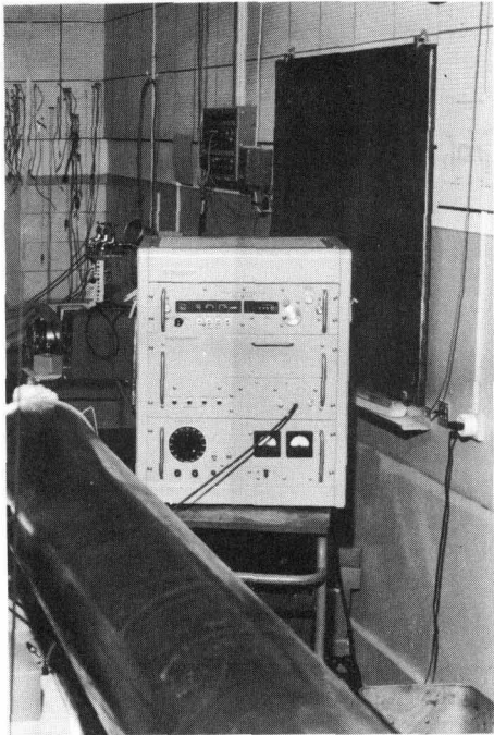
Fig. 5. Frequency comparison being made between one standard and the "long" cesium beam standard (foreground) at the Laboratoire Suisse de Recherches Horlogeres, Neuchatel, Switzerland. This long standard is considered one of the world's best cesium standards.
