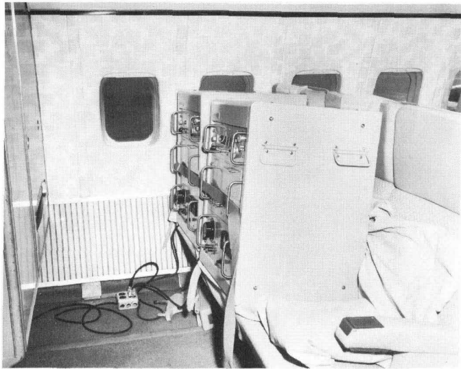
Fig. 2. The two atomic clocks being fastened in passenger seats aboard airliner. Operating power in flight was supplied by plane.
